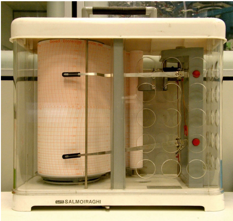
Abb. 2: Hygrograph
