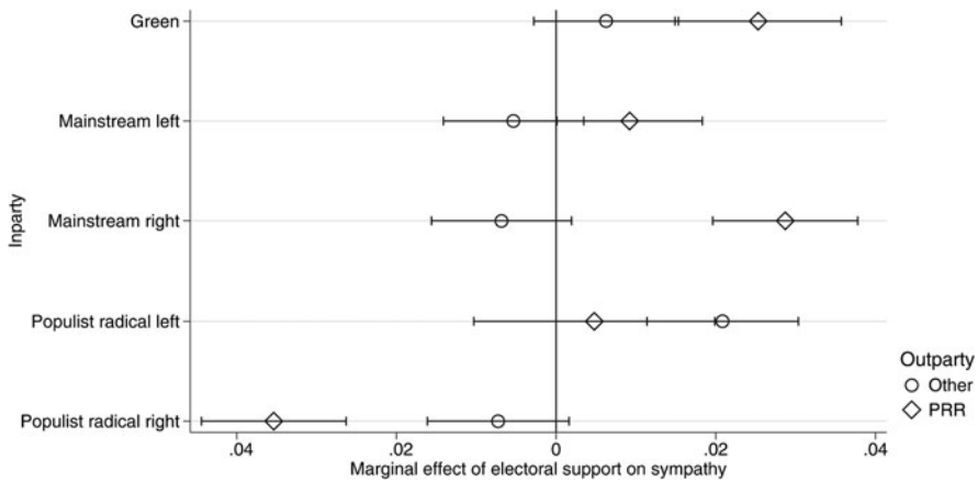
Figure 3. Marginal Effect of Electoral Support for a Party (in %) on Sympathy for that Party, by PRR v. Other
