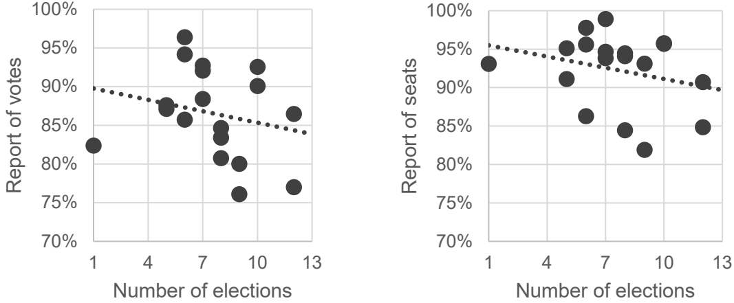
Figure 2. Voting and seats reported according to number of elections
