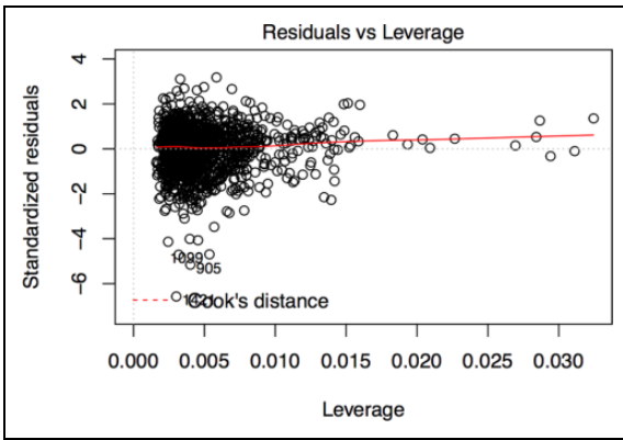
Figure 10. Standardized residuals versus leverage measure.
