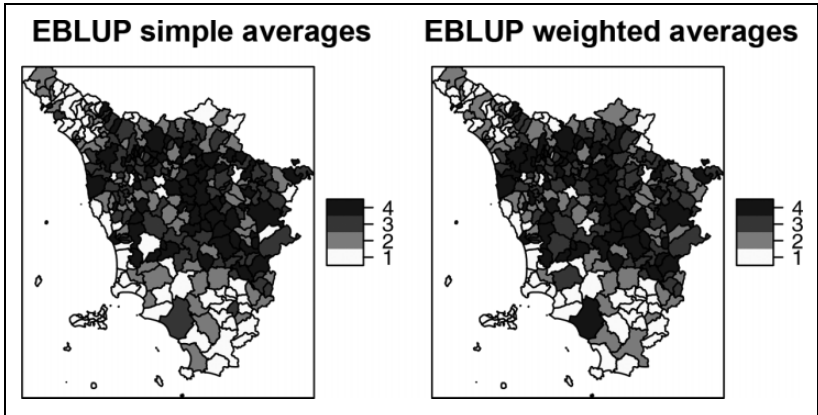
Figure 8. Latent economic well-being indicator based on simple and weighted averages of single empirical best linear unbiased predictions (1 = first quartile, 2 = second quartile, 3 = third quartile, 4 = fourth quartile).
