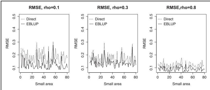
Figure 2. Root mean squared error for direct estimates and empirical best linear unbiased prediction of factor score means for small areas with n_d > 0 .
