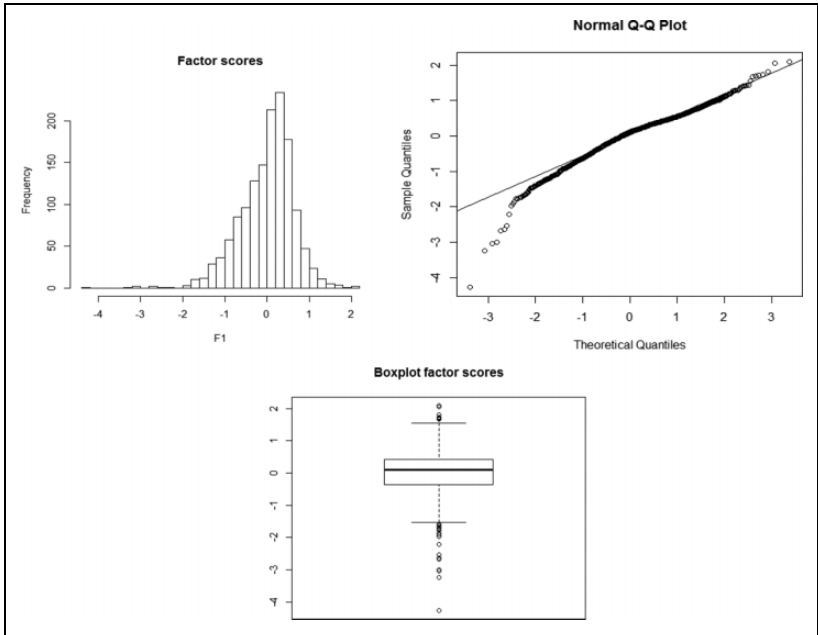
Figure 5. Factor scores distribution graphs.
