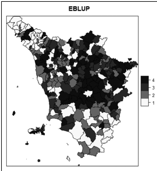
Figure 7. Latent economic well-being indicator based on transformed empirical best linear unbiased prediction of factor scores means (1 = first quartile, 2 = second quartile, 3 = third quartile, 4 = fourth quartile).
