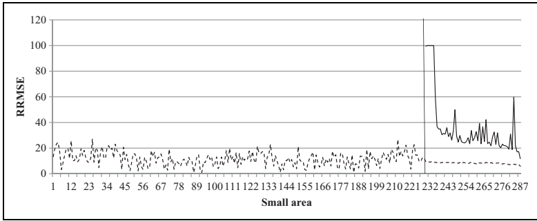
Figure 6. Relative root mean squared error direct estimates (—) and empirical best linear unbiased predictions (---) ordered by growing sample size.
