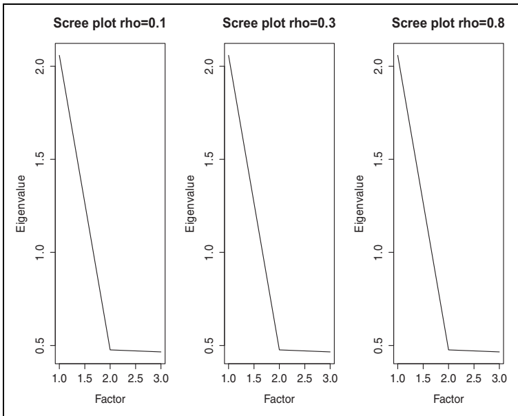
Figure 1. Scree plots from the explanatory factor analysis of the simulation population.
