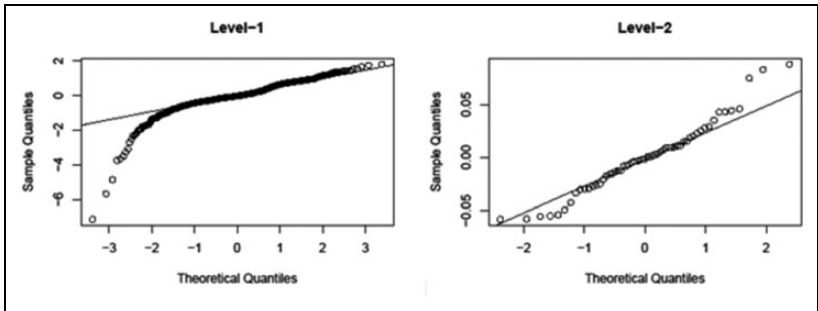
Figure 9. Q–Q plots for the level 1 and level 2 residuals of the Battese, Harter, and Fuller model fitting.
