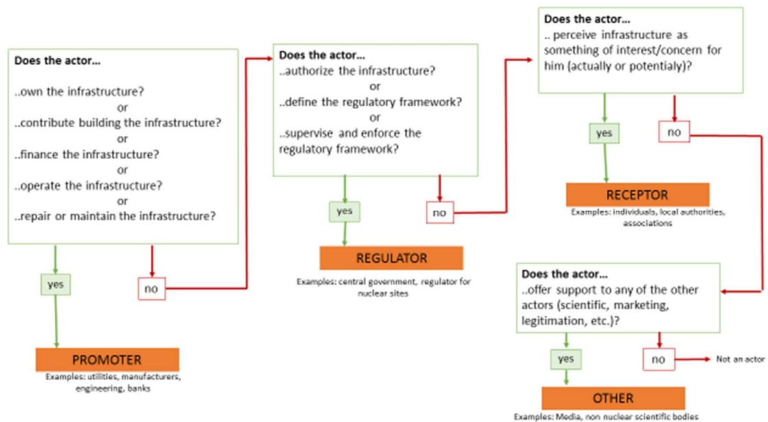
Figure 1: Actor's taxonomy
