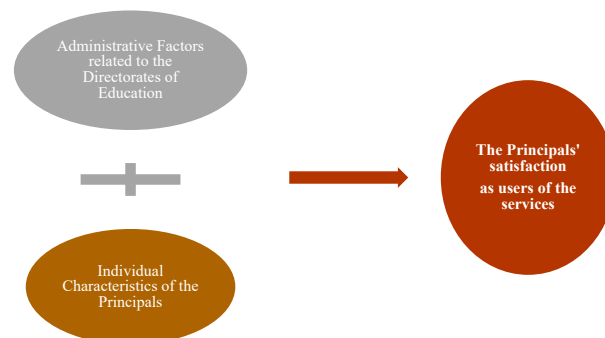
Figure 1. Theoretical Framework
