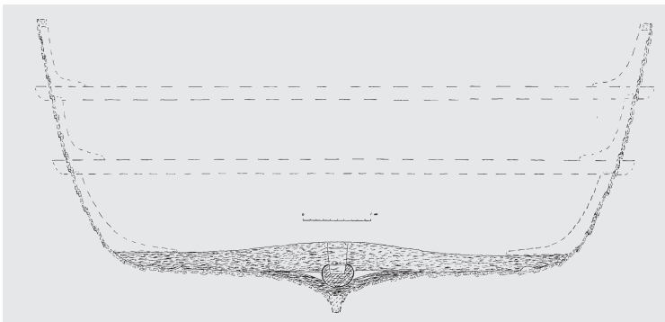
Fig. 3 Rough sketch reconstruction of the cross section of the Big Ship at the mast. (Drawing: A.E. Christensen)
