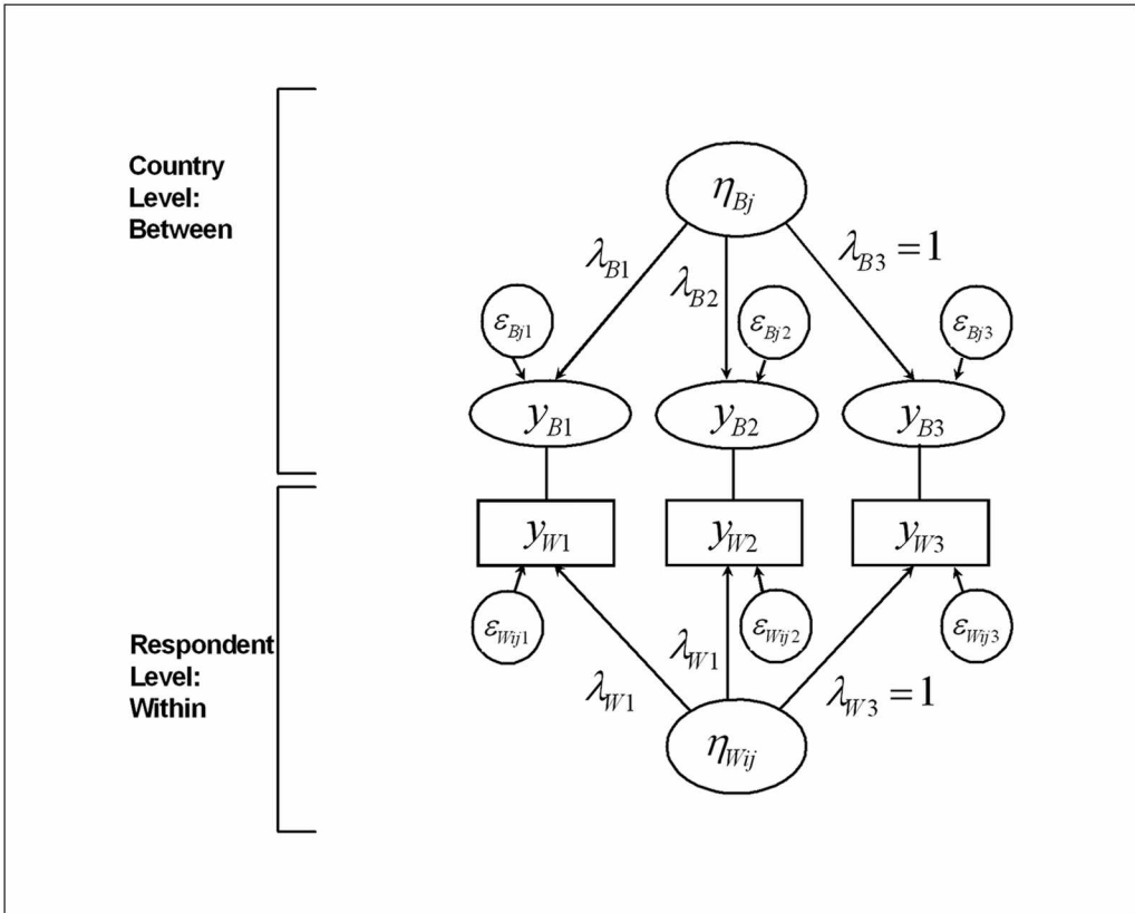
Figure 1. A Two-Level CFA With Three Indicators
