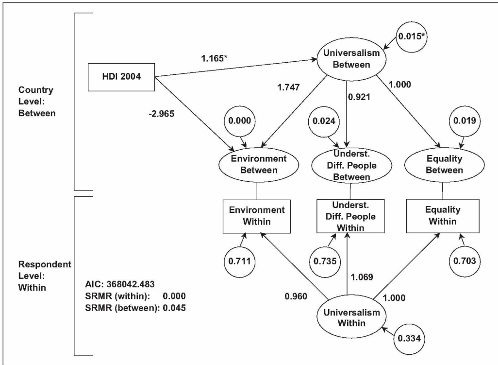
Figure 2b. A Multilevel SEM for Universalism (Model 2)
