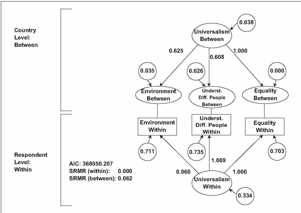
Figure 2a. A Multilevel CFA for Universalism (Model 1)
