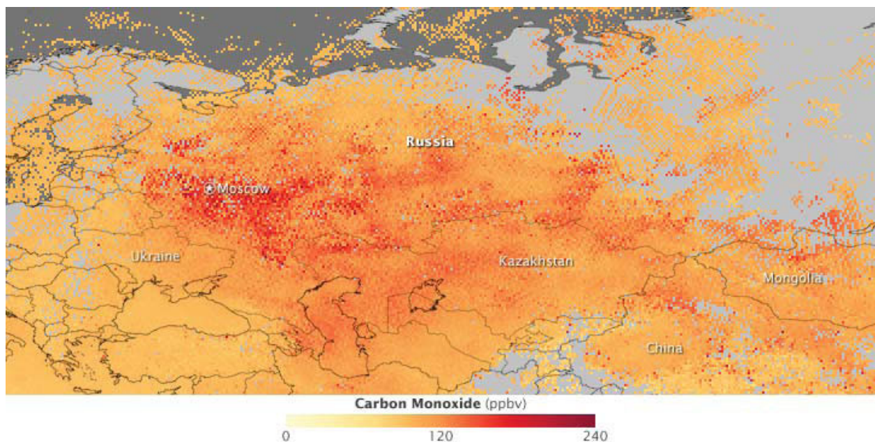
Figure 2. Carbon monoxide concentrations in the atmosphere between 2 and 8 km above Russia as recorded from 1 to 8 August 2010. Ground concentrations of this dangerous gas are reported to be much higher, causing people to report headaches, dizziness, and other more serious conditions. Source: NASA MOPITT.
