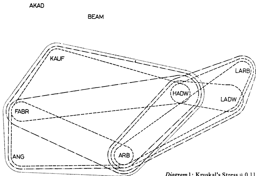
Diagram 1: Kruskal's Stress = 0.115
