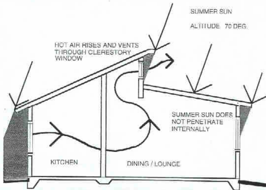
Figure 2 Typical section showing summer conditions
