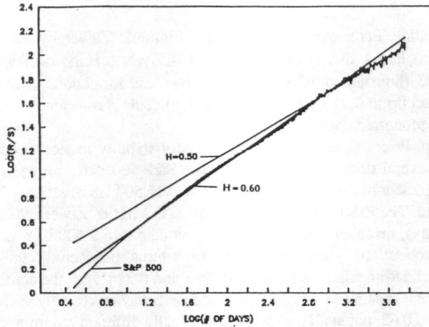
R/S analysis: S&P 500 daily returns, January 2, 1928–December 31, 1989. Estimated H=0.60 . Note the cycle length of 1,000 trading days, or about four years, which we also saw in the monthly analysis in Figure 8.3.
