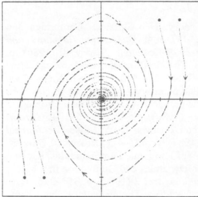
Fig. 2: Attractors
