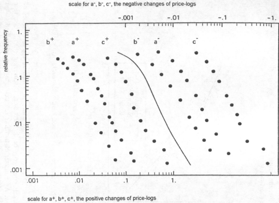
Fig. 7: Scale Invariance
