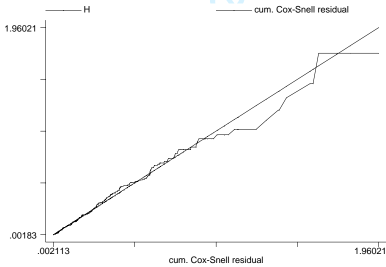
Figure 7: Cox-Snell Residuals for Weibull Model
