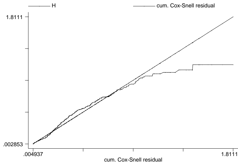
1 2 3 4 5 Figure 4: Cox-Snell Residuals, Log-logistic model, smokers and non-smokers 6 7 8
