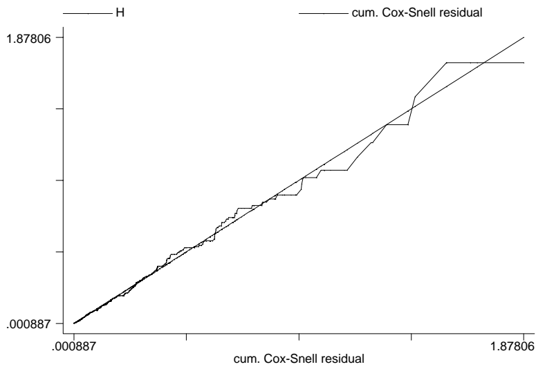
Figure 6: Cox-Snell Residuals for Gamma Model
