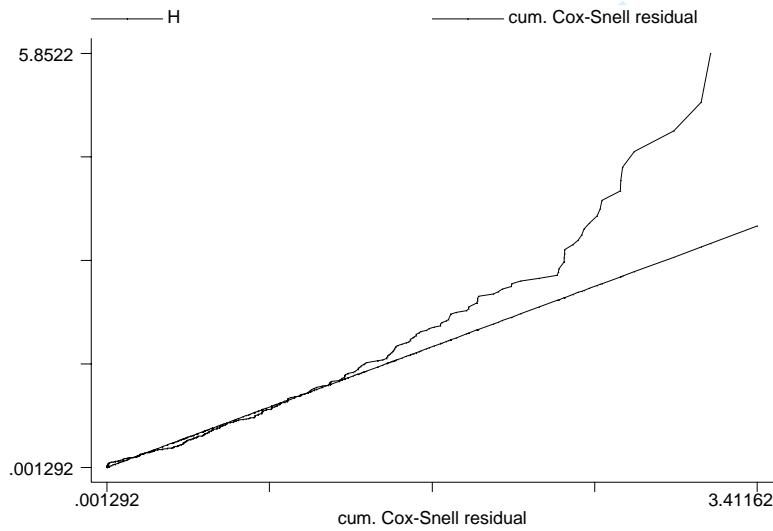
Figure 3: Cox-Snell Residuals, Log-logistic model, smokers only
