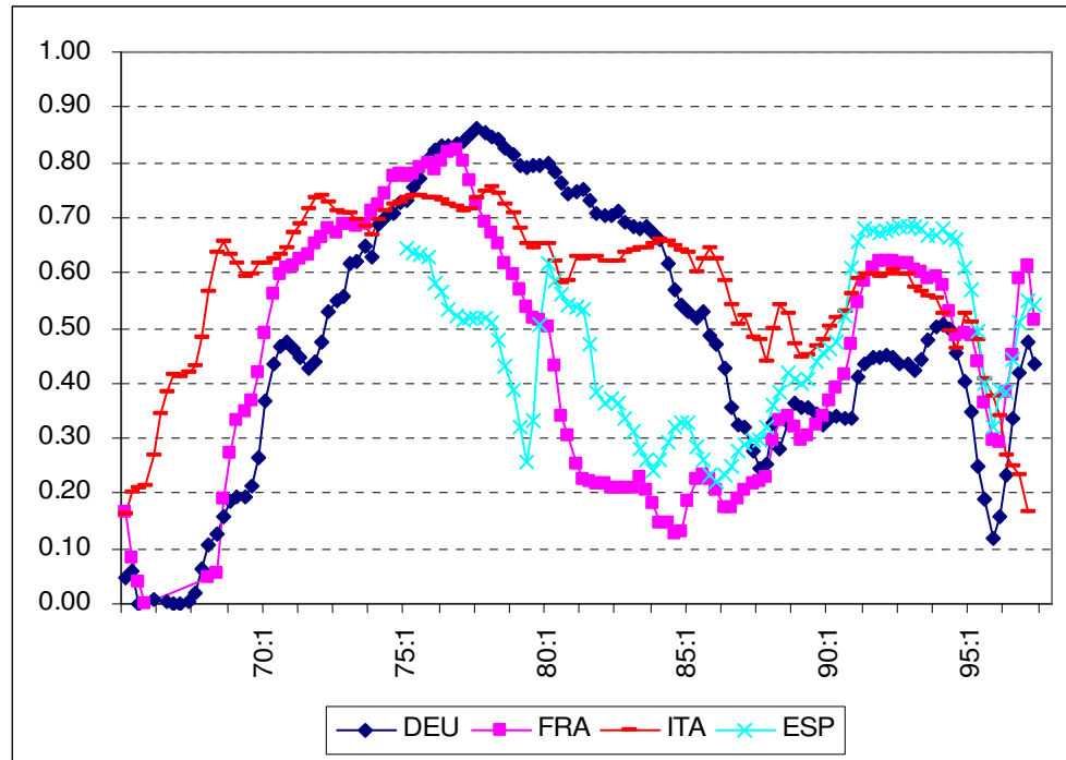
Figure 4: Maximum positive rolling correlation of HP detrended GDP with respect to the US
