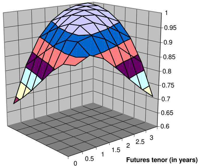
Model implied instantaneous correlations
