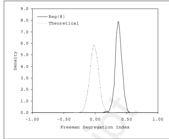
Figure 11: FSI levels generated by the model (solid line) v. FSI Simulated Theoretical Distribution (dashed line). Network: Regular lattice with d = 8 . Parameters: M = 100 , \theta = 0.3 . Sample Sizes: Model = 1000; Simulated Index Distribution = 100,000.
