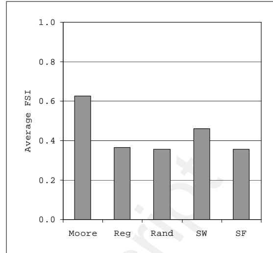
Figure 7: Average Freeman’s Segregation Index (FSI) v. Network Classes. Average Degree d = 8 . Parameters: M = 100 , \theta = 0.3 . MC Sample Size = 1000.
