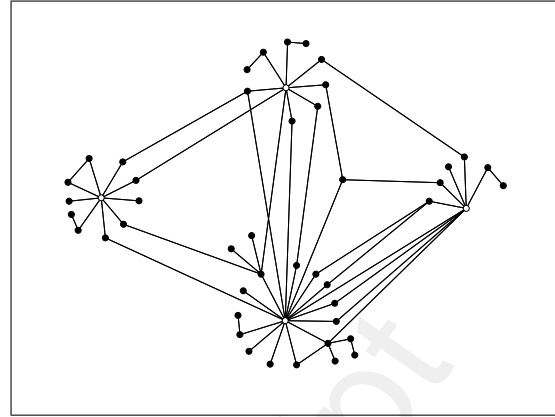
Figure 5: An example of a scale-free graph obtained applying a preferential attachment algorithm. The initial population size is M_0 = 16 . Final population size is M = 100 . All initial nodes have degree d = 4 . White nodes are the “hubs”.
