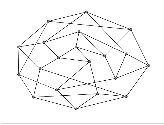
Figure 2: An example of a regular graph with degree d = 4 and M = 20 nodes. Notice how all nodes hold exactly 4 links.
