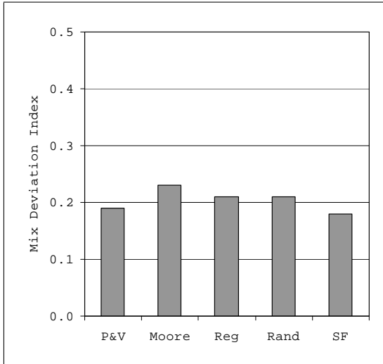
Figure 12: Average Mix Deviation Index v. Network Classes. Average Degree d = 8 . Parameters: M = 100 , \theta = 0.2 . MC Sample Size = 1000. PV: Average values reported in Pancs and Vriend (2003) for the case 2D-M without boundaries and same parameter values.
