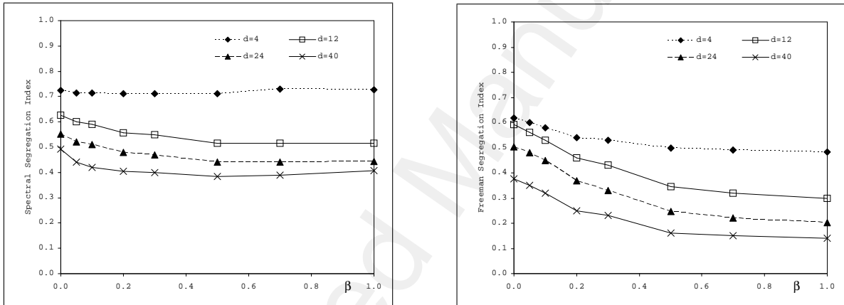
Figure 16: Small-World Networks. SSI (left) and FSI (right) v. different rewiring probabilities \beta and alternative average degrees. Parameters: M = 100 , MC Sample Size: 1000
