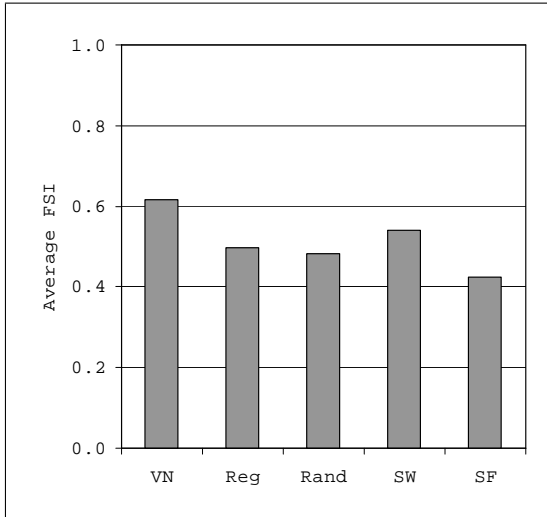
Figure 6: Average Freeman’s Segregation Index (FSI) v. Network Classes. Average Degree d = 4 . Parameters: M = 100 , \theta = 0.3 . MC Sample Size = 1000.
