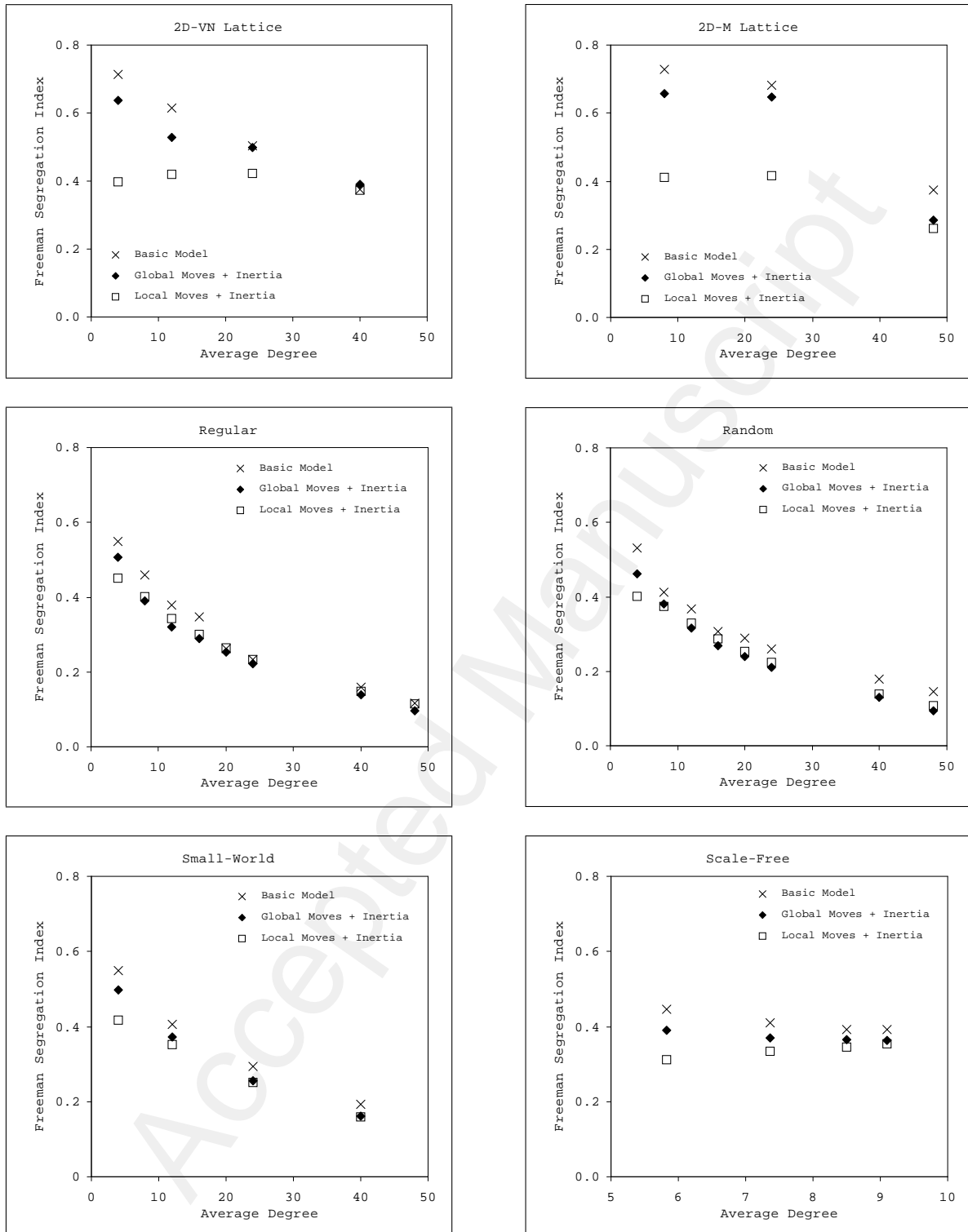
Figure 18: FSI v. Average Degree in three alternative setups: (i) Basic Model; (ii) Inertia in individual decision rules; (iii) Inertia in individual decision rules and local moves. See Section 5.3 for details. Parameters: M = 100 , \theta = 0.3 , MC Sample Size: 1000
