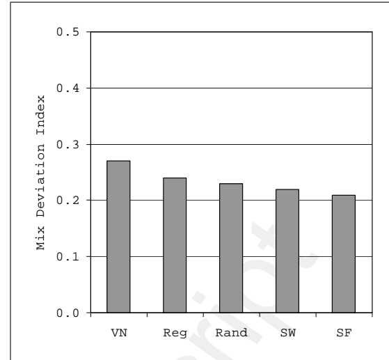
Figure 13: Average Mix Deviation Index v. Network Classes. Average Degree d = 4 . Parameters: M = 100 , \theta = 0.2 . MC Sample Size = 1000.
