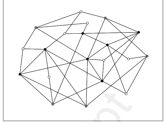
Figure 3: An example of a random graph with average degree d = 4 and M = 20 nodes. Nodes color depends on node degree. Black nodes: d > 4 . Grey nodes: d = 4 . White nodes: d < 4 .
