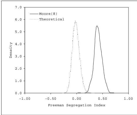
Figure 10: FSI levels generated by the model (solid line) v. FSI Simulated Theoretical Distribution (dashed line). Network: 2D-M lattice with r = 1 ( d = 8 ). Parameters: M = 100 , \theta = 0.3 . Sample Sizes: Model = 1000; Simulated Index Distribution = 100,000.
