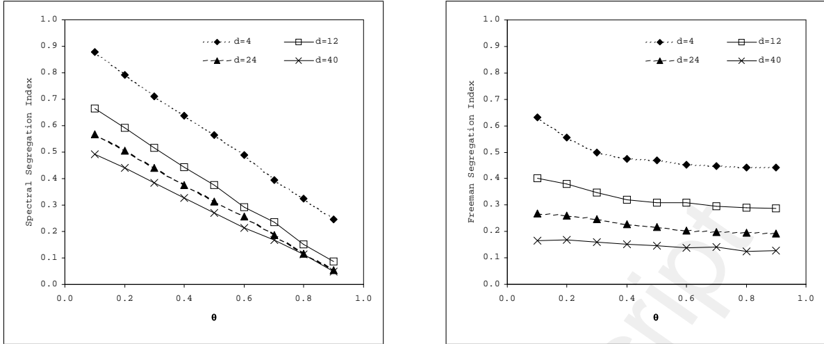
Figure 15: Small-World Networks. SSI (left) and FSI (right) v. \theta for Different Average Degrees. Parameters: M = 100 , MC Sample Size: 1000
