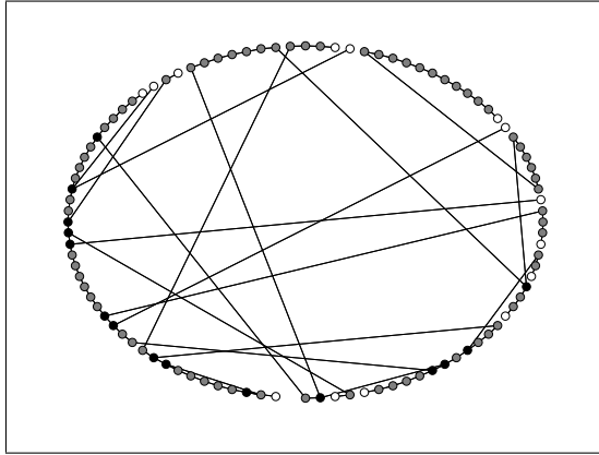
Figure 4: An example of a small-world graph obtained from M = 100 nodes originally lying on a circle and interacting with their nearest neighbors only ( r = 1 ). Rewiring probability \beta = 0.2 . Nodes color depends on degree after rewiring. Black nodes: d \geq 3 . Grey nodes: d = 2 . White nodes: d = 1 .
