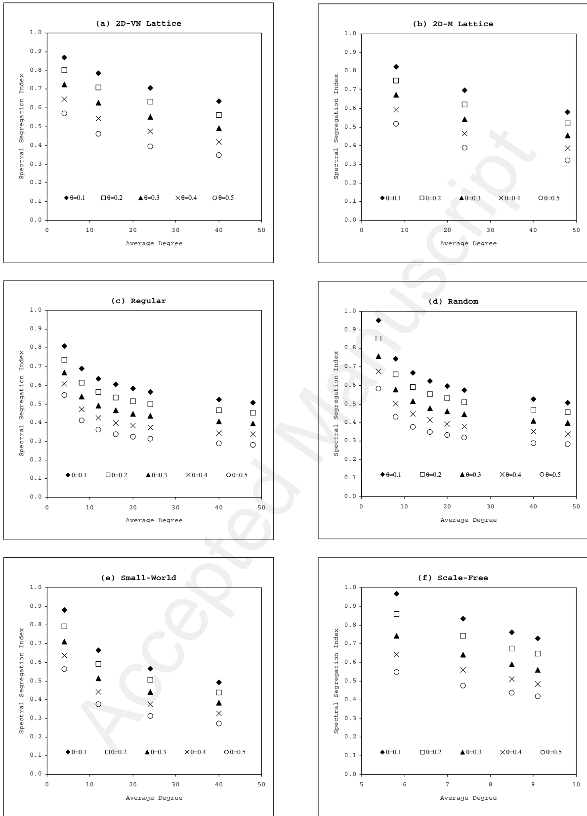
Figure 14: SSI v. Average Degree for Different Levels of \theta . Parameters: M = 100 , MC Sample Size: 1000
