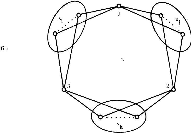
Figure 4. A Graph G , All 2-clubs Are 2-clans
