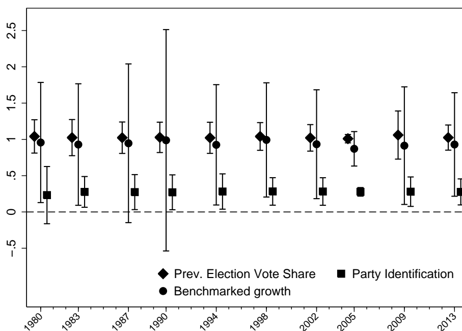
Figure 2: Stability of coefficient estimates
