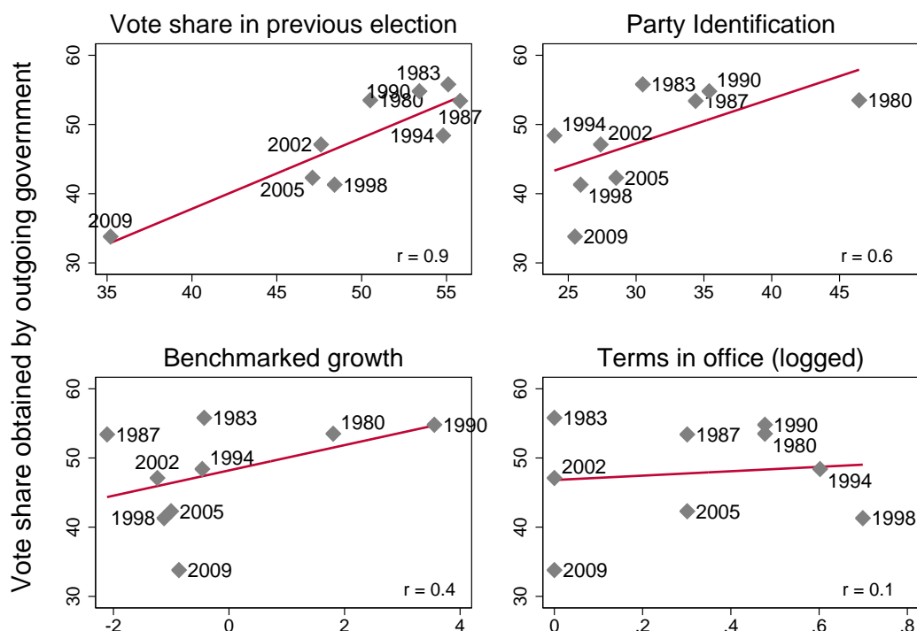
Figure 1: Predictors of the vote
