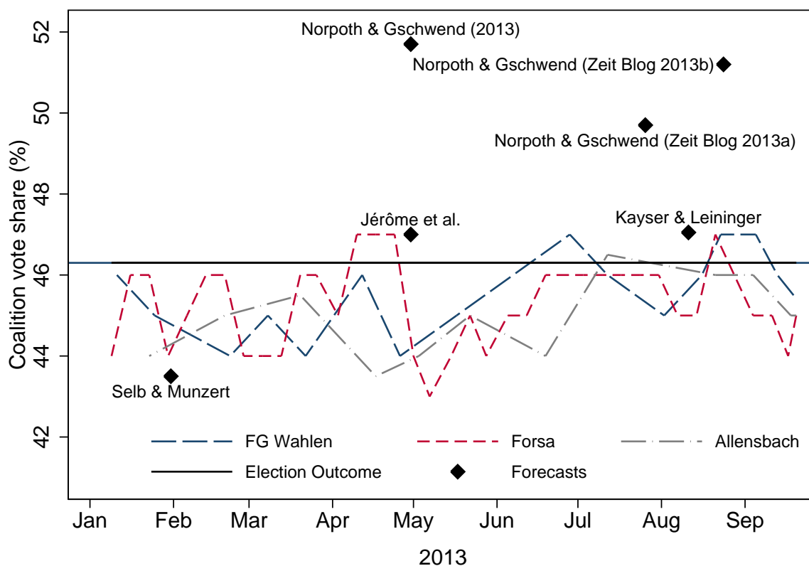
Figure 4: Timeline of election forecasts
