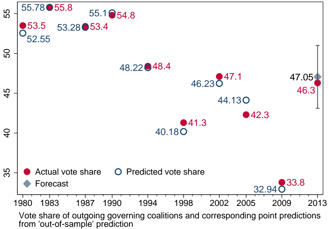
Figure 3: Actual and predicted vote share
