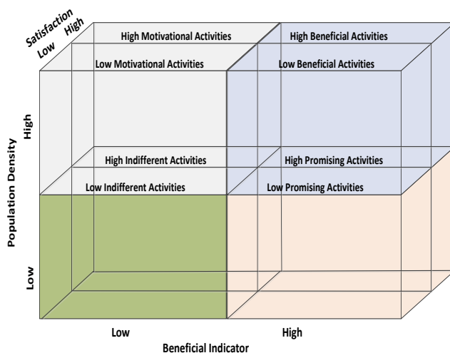
Figure 2: TiCoSa Model
