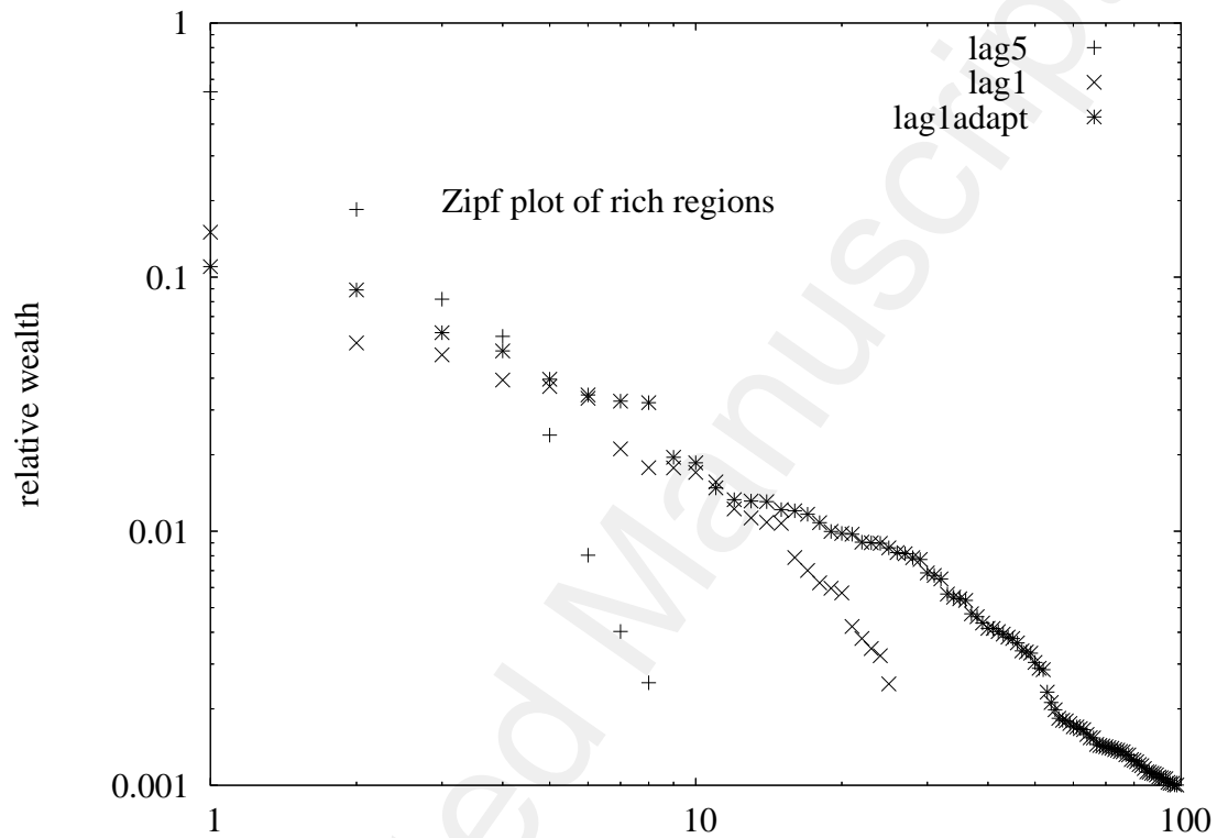
Figure 8: Zipf plot of wealth of the most active regions for the standard and adaptive firms models (cf. section 4.1). The vertical axis displays the production relative to the total production. The '+' signs correspond to the standard model with time lag = 5, the 'x' to time lag = 1, and the '*' to the adaptive firms model with time lag = 1.
