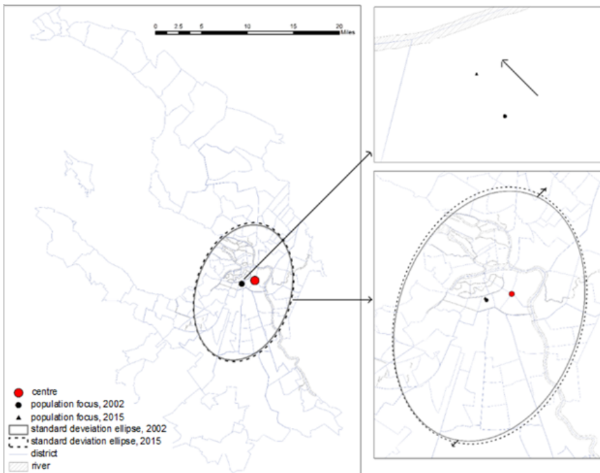
Fig. 5. Spatial changes in the centre of gravity and standard deviation ellipse in 2002—2015
