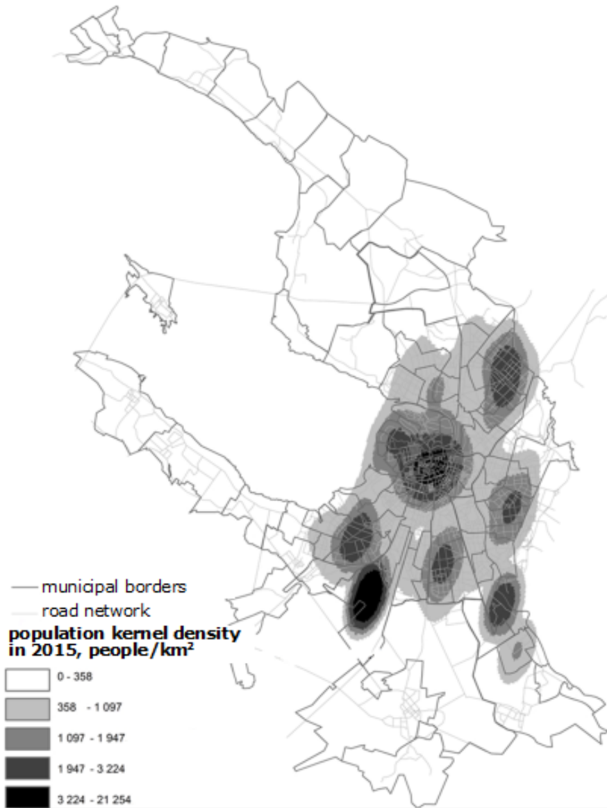
Fig. 12. Kernel density in Saint Petersburg, 2015 (KDE)
