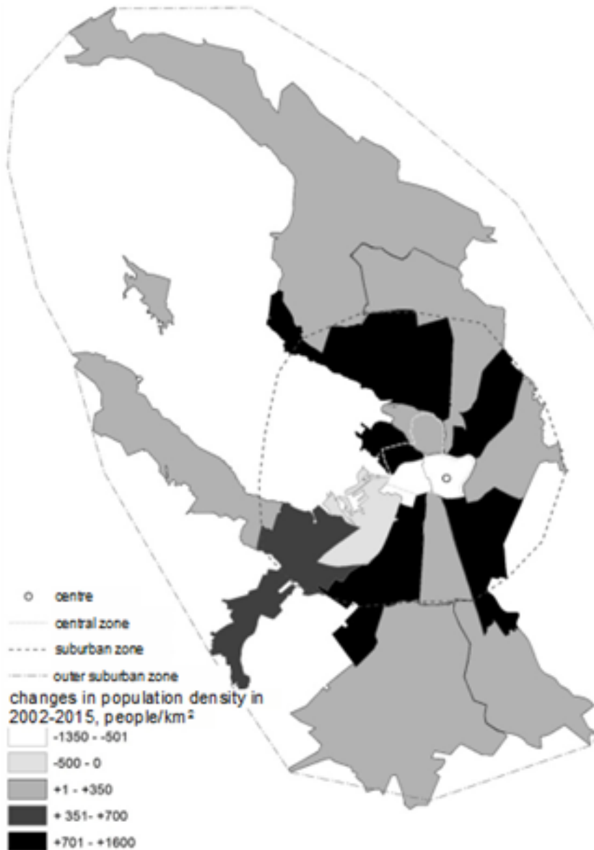
Fig. 4. Changes in population density in Saint Petersburg districts in 2002—2015
