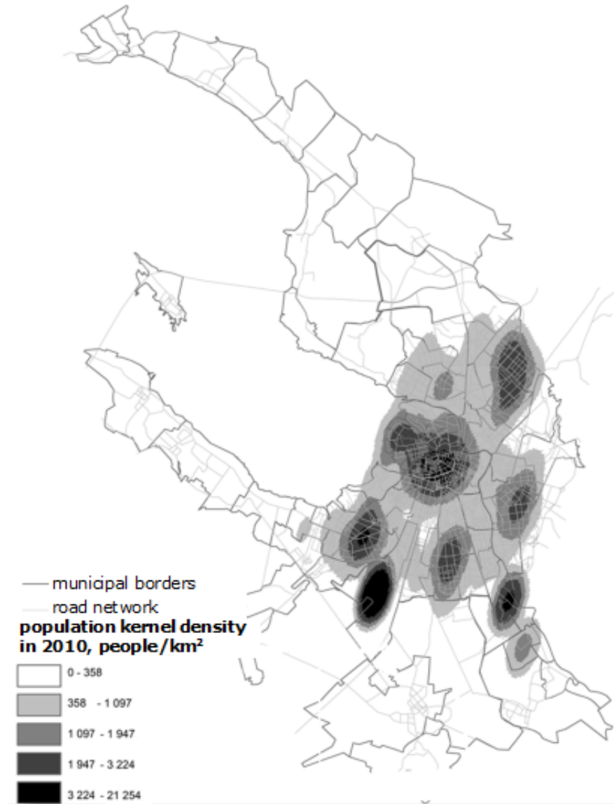
Fig. 11. Kernel density in Saint Petersburg in 2010 (KDE)
