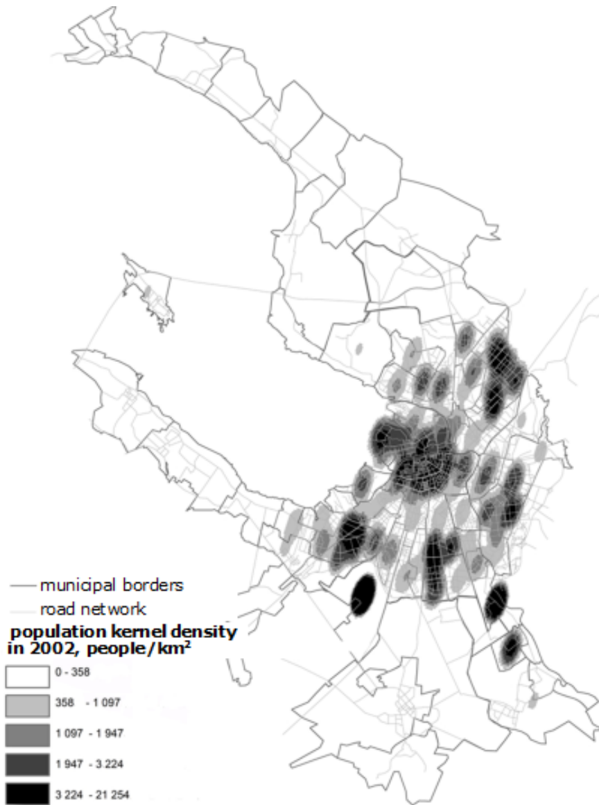
Fig. 10. Kernel density in Saint Petersburg in 2002 (KDE)
