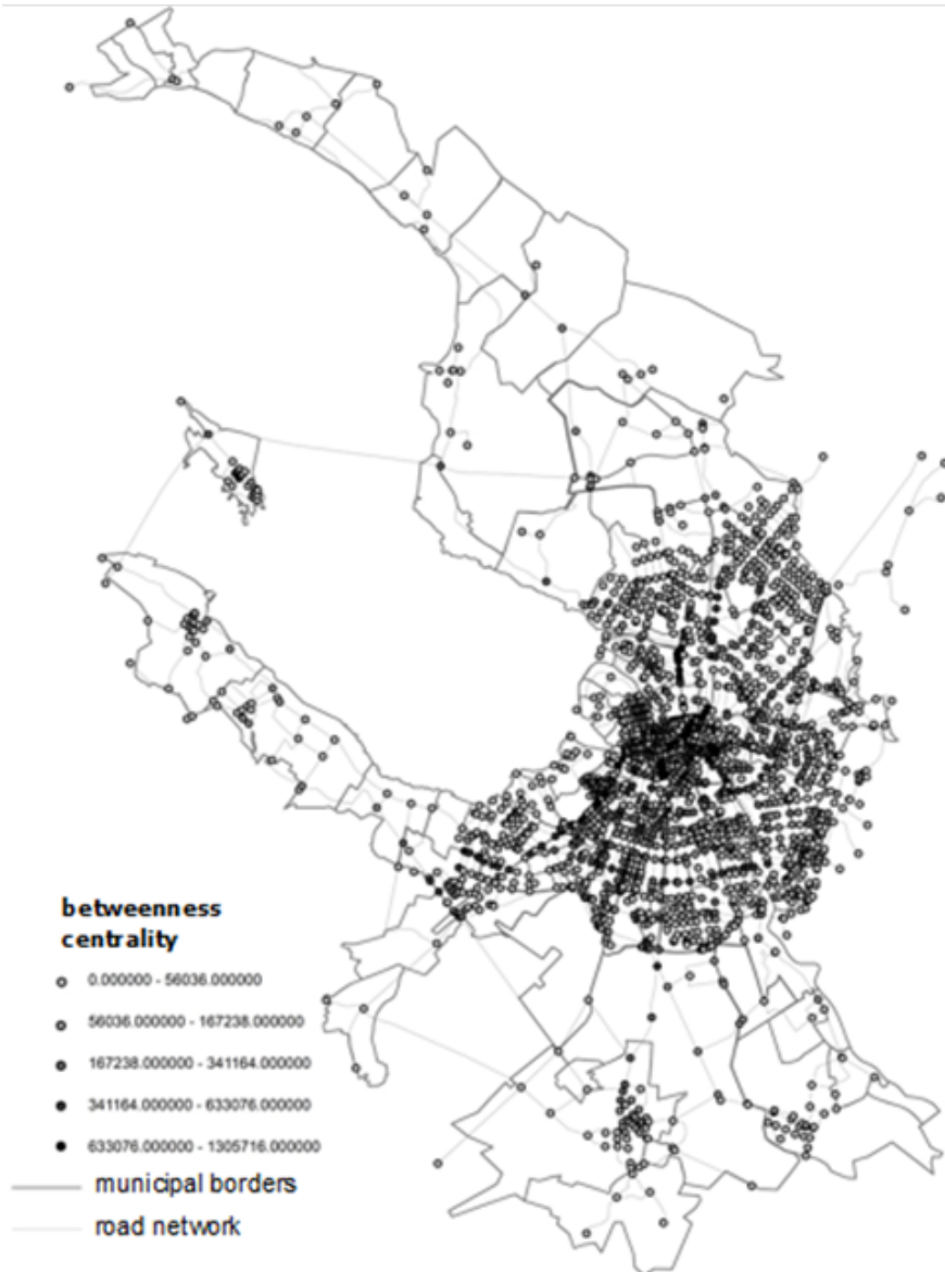
Fig. 6. Betweenness centrality of Saint Petersburg transport network zones
