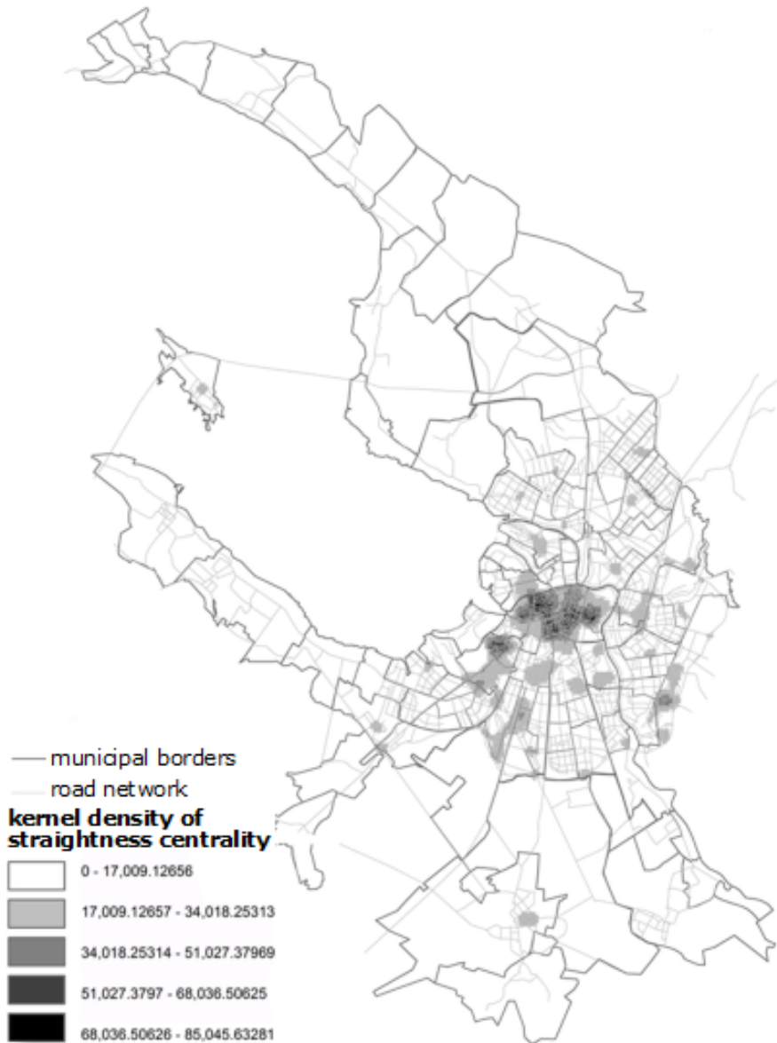
Fig. 9. Kernel density of straightness centrality of Saint Petersburg transport network (KDE)
