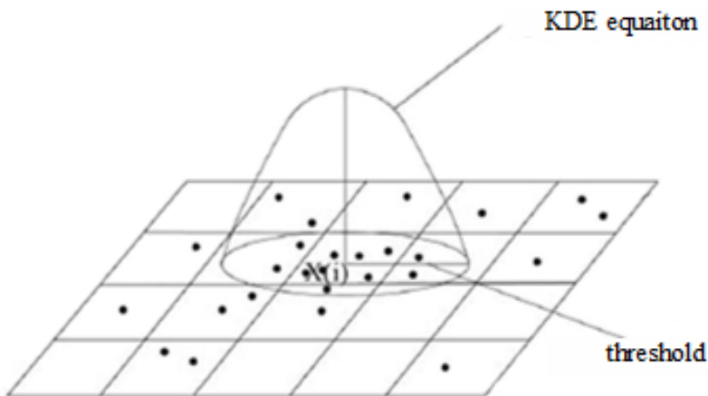
Fig. 1. Kernel density estimation method
